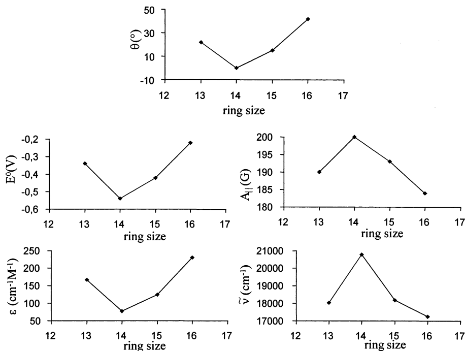
Fig. 8. Correlation of the CuN 4 plane twist angle \theta (see Chart 3), the reduction potential E^\circ , the EPR hyperfine parameter A_{||} , the d–d transition \nu_1 and its extinction coefficient \epsilon_1 with the macrocycle ring size [54,57,176].
